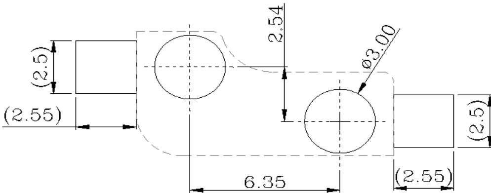
PCB LAYOUT
